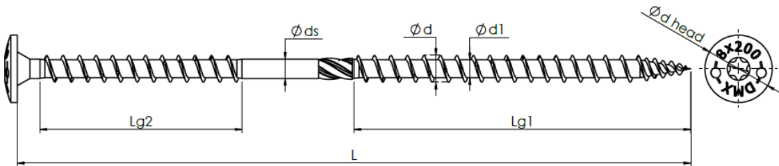
Figure 3: Screw, type WKT
