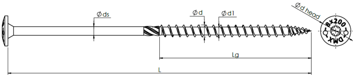
Figure 2: Screw, type CT
