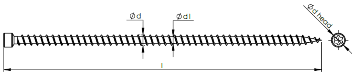
Figure 5: Screw, type CPW
