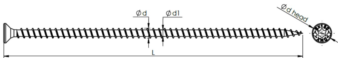
Figure 6: Screw, type CPS
