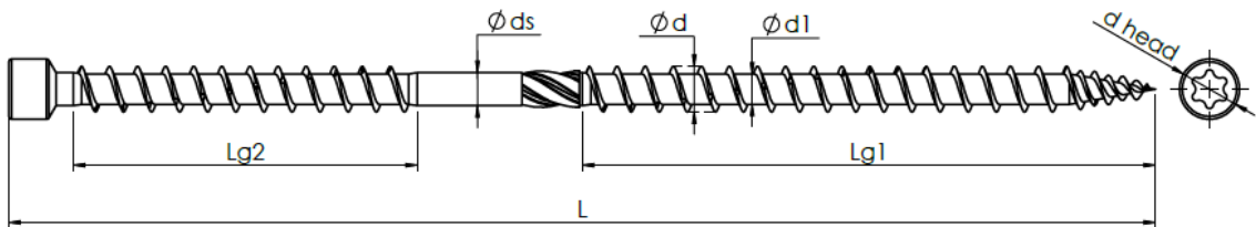
Figure 4: Screw, type WKW
