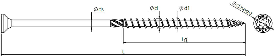
Figure 1: Screw, type CS
