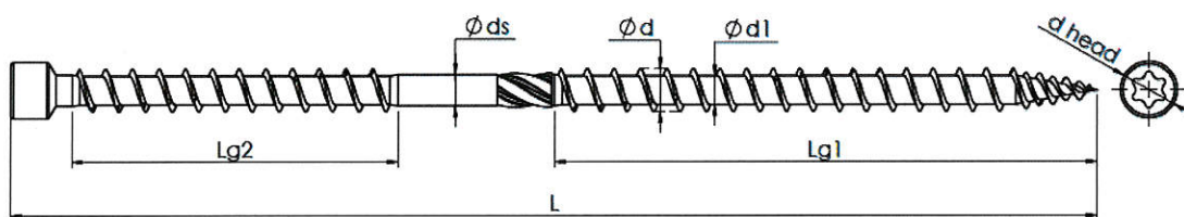
Figure 4: Screw, type WKW
