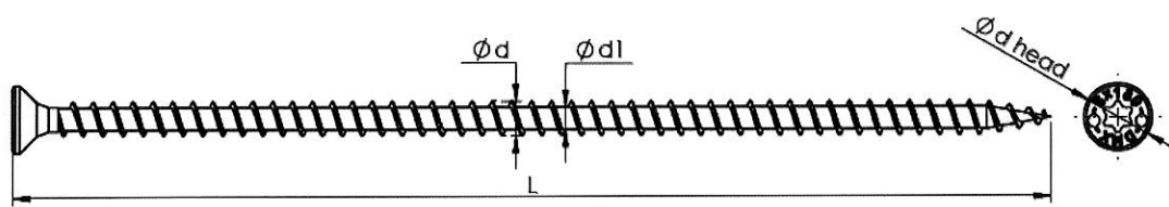
Figure 6: Screw, type CPS
