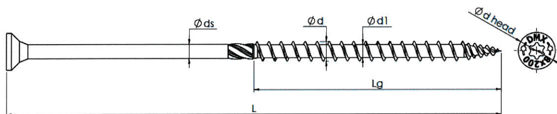
Figure 1: Screw, type CS
