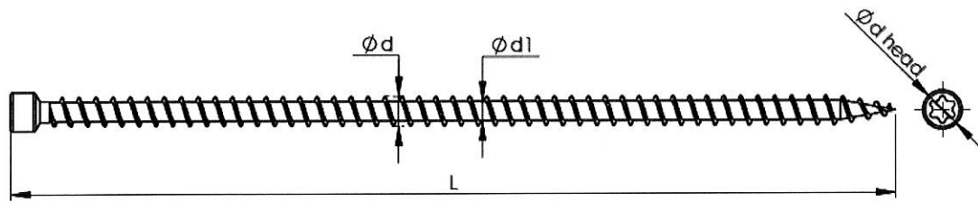
Figure 5: Screw, type CPW
