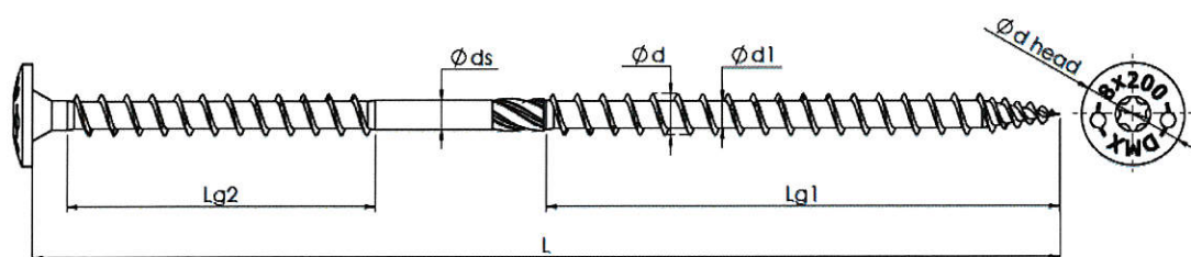
Figure 3: Screw, type WKT
