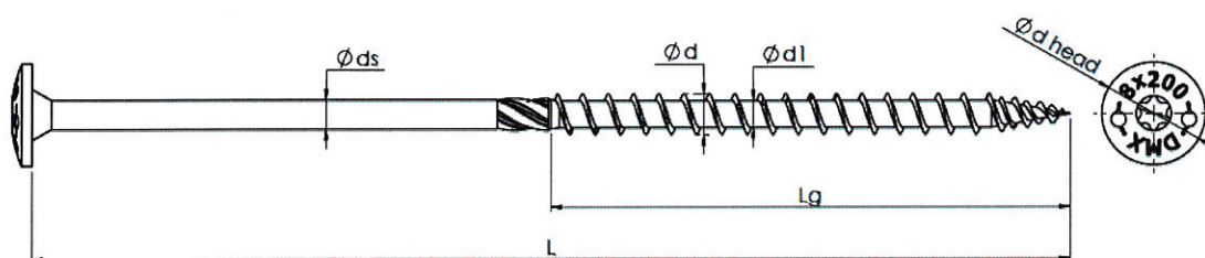
Figure 2: Screw, type CT
